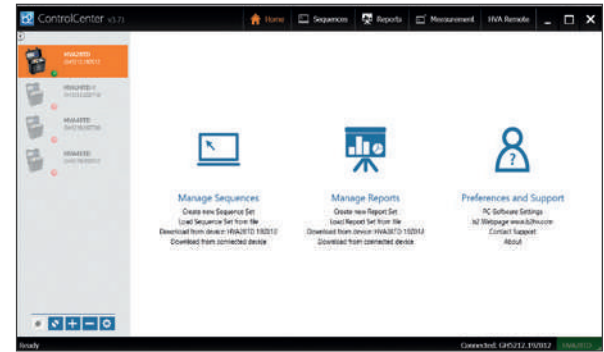
User interface
