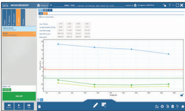
TD over voltage chart
